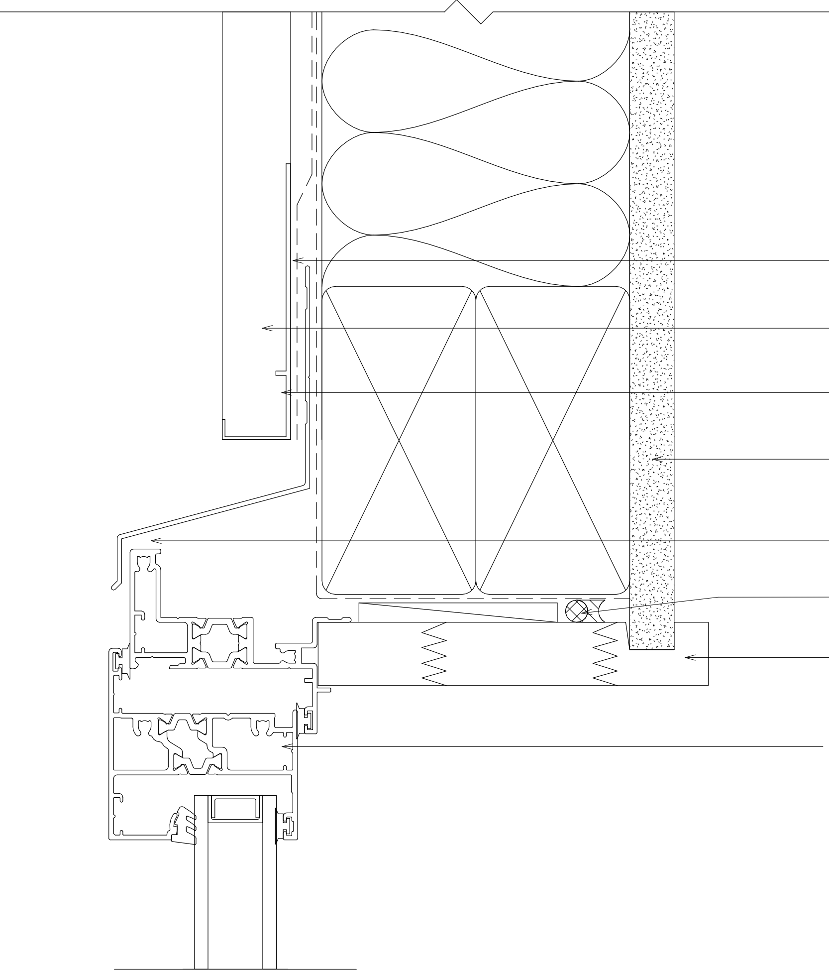
FLASHING TAPE TO LAP HEAD FLASHING AS PER E2AS1 CAVITY BATTEN CAVITY CLOSER INTERNAL LININGS EXTRUDED ALUMINIUM HEAD FLASHING PEF ROD AND AIR SEAL TIMBER LINER 801 AWNING WINDOW
